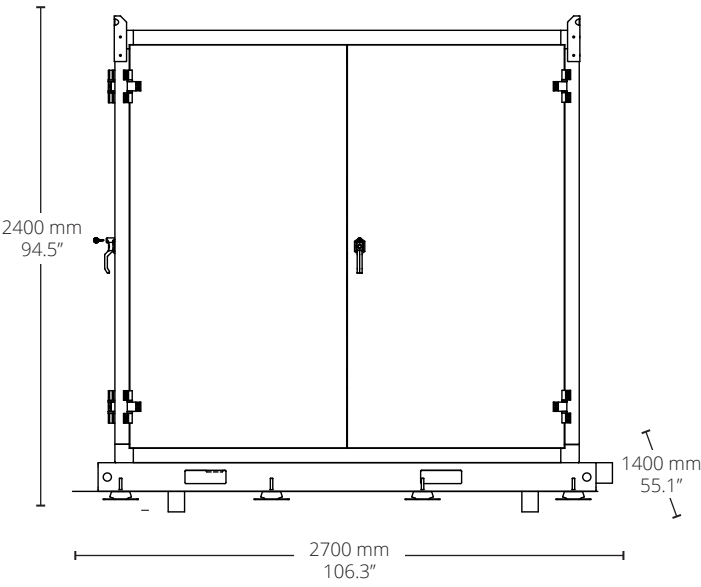
(Fig. B) Outdoor Unit Enclosed available in standard or low-noise versions
